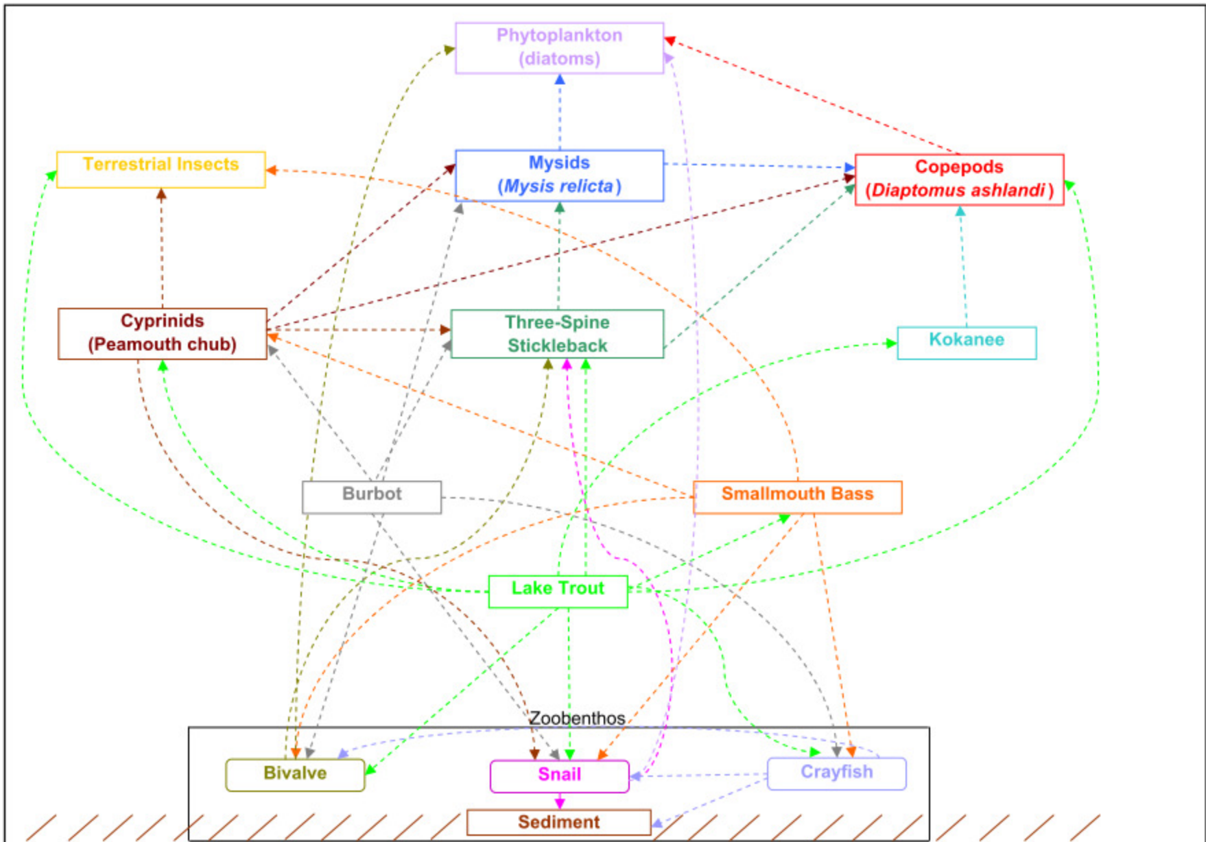
CONCEPTUAL DIAGRAM SHOWING ORGANISMS INCLUDED IN THE LAKE CHELAN CONTAMINANT FOOD WEB MODEL WRIA 47 Phase II Watershed Planning Chelan County, Washington By: sge Date: 06/22/09 Project No. 13462.002 AMEC Geomatrix Figure 1
